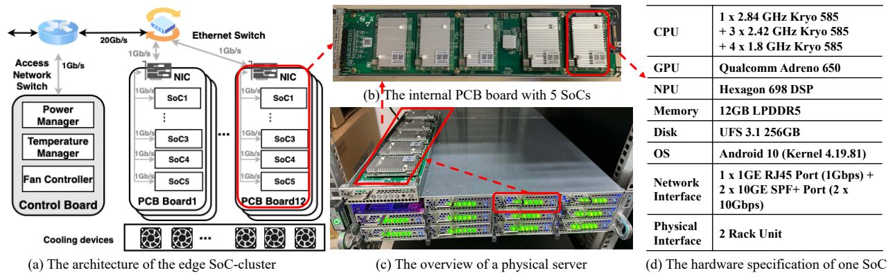
Figure 2. The overview of a typical edge SoC-Cluster that has been widely deployed in a real environment.
